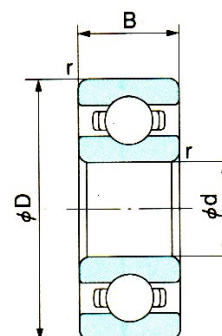
Illustration 1: Bearing Dimensions
